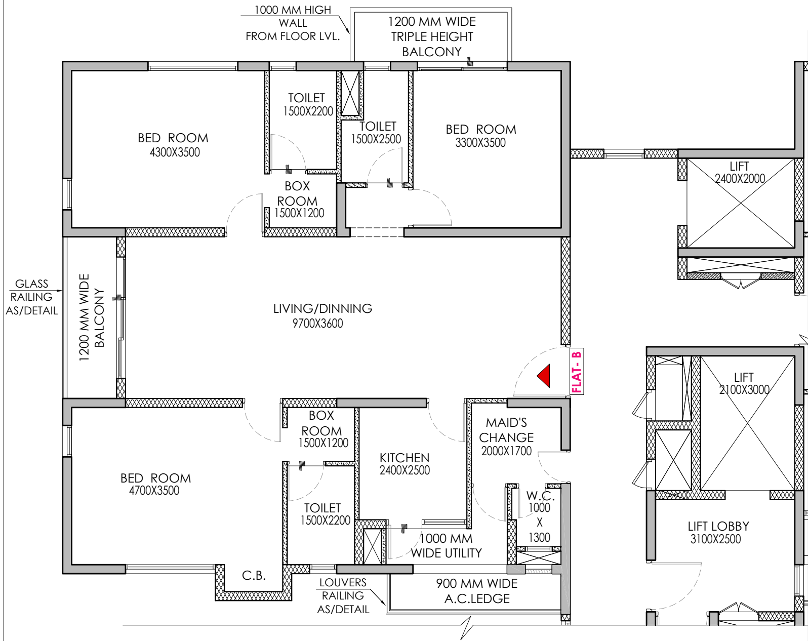
FLAT-B 4TH FLOOR PLAN (7TH, 10TH, 13TH, 16TH, 19TH, 22TH, 25TH & 28TH FLOOR) N
