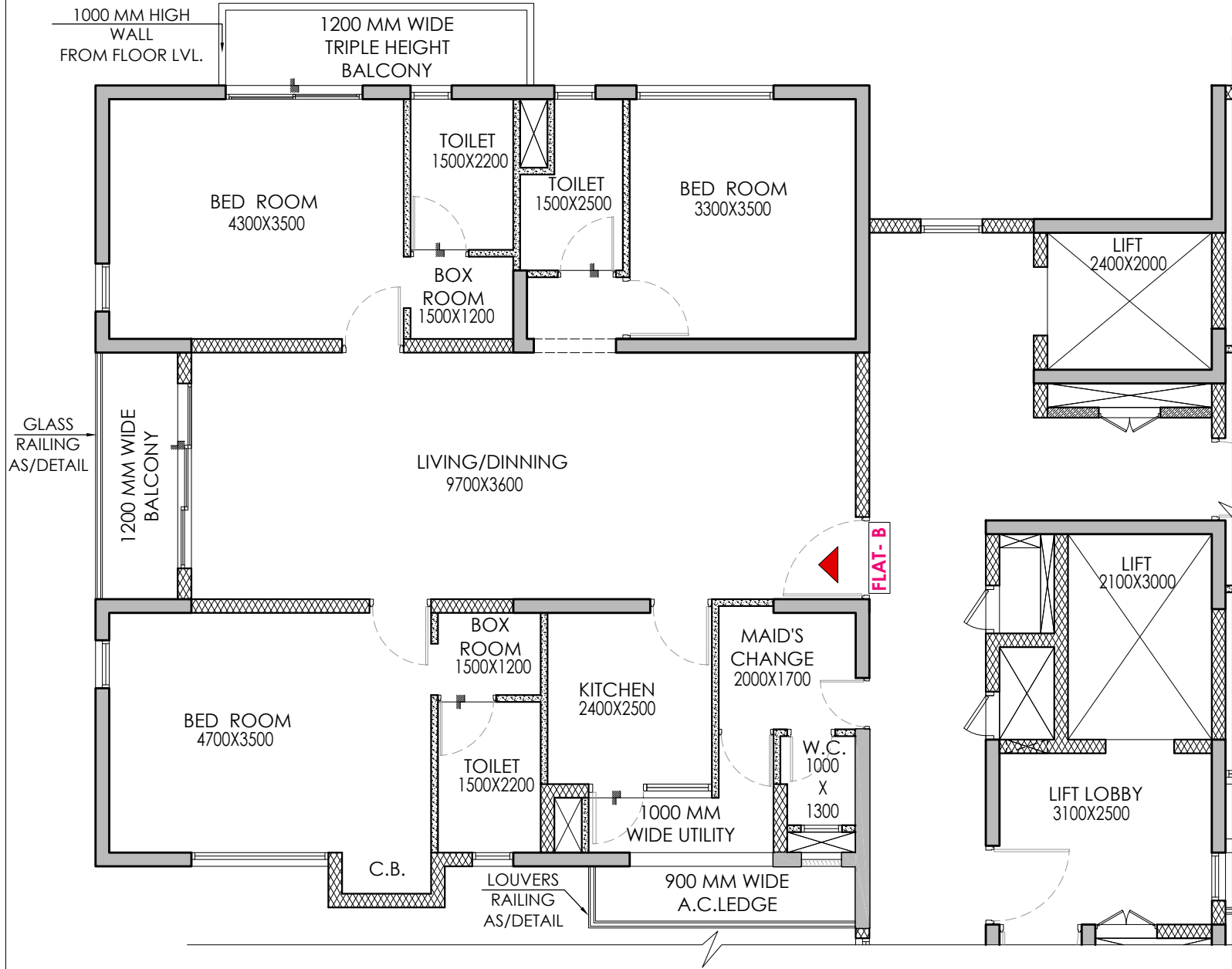
FLAT-B 3RD FLOOR PLAN (6TH, 9TH, 12TH, 15TH, 18TH, 21TH, 24TH, 27TH & 30TH)
