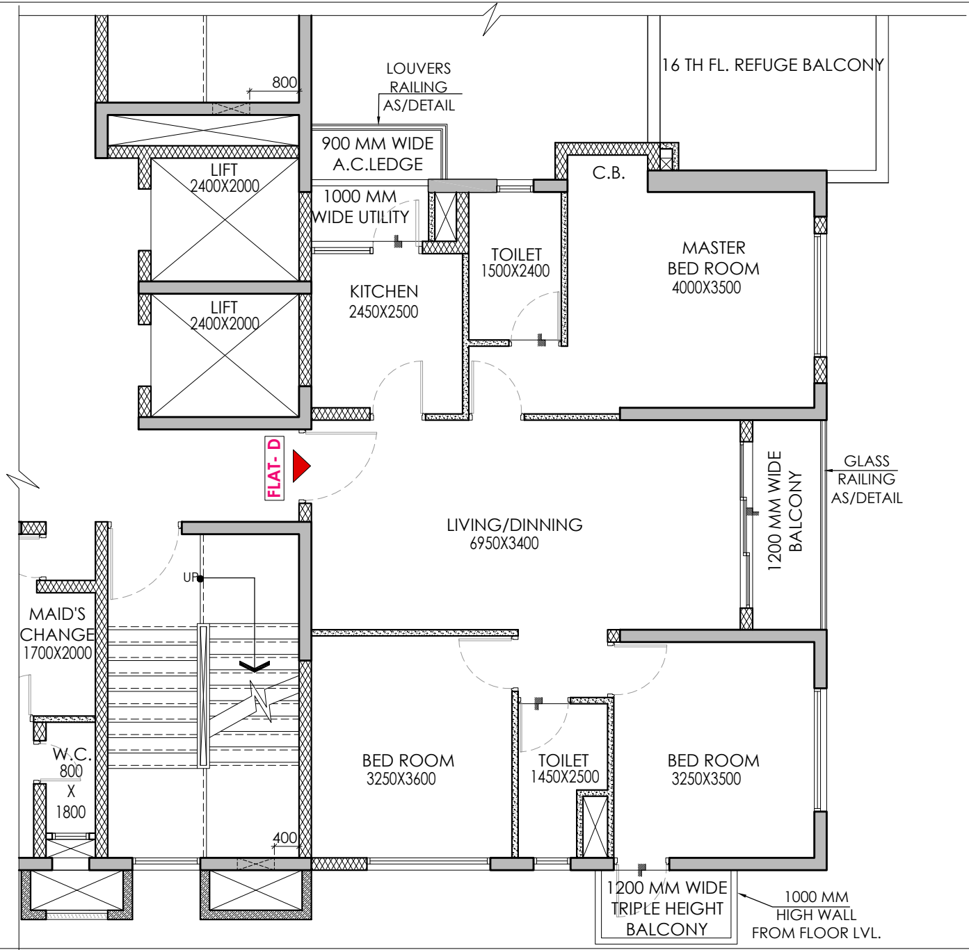
FLAT-D 4TH FLOOR PLAN (7TH, 10TH, 13TH, 16TH, 19TH, 22TH, 25TH & 28TH FLOOR)
