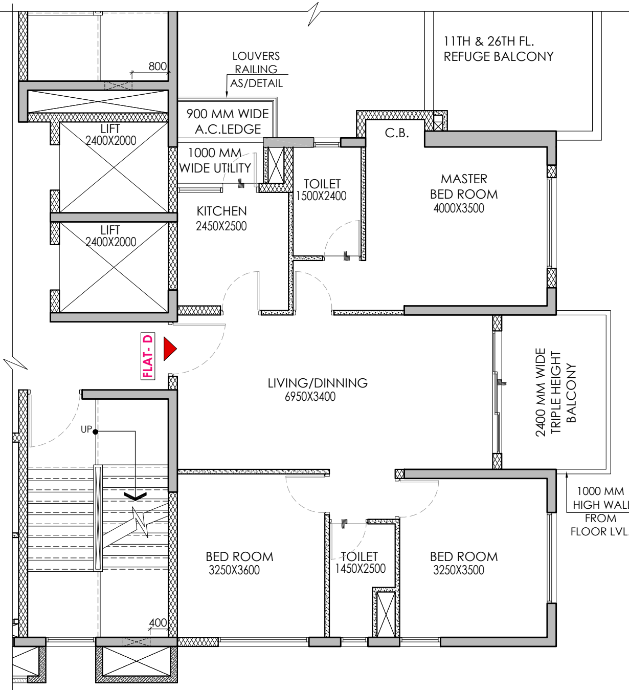
FLAT-D 5TH FLOOR PLAN (8TH, 11TH, 14TH, 17TH, 20TH, 23TH, 26TH & 29TH FLOOR)
